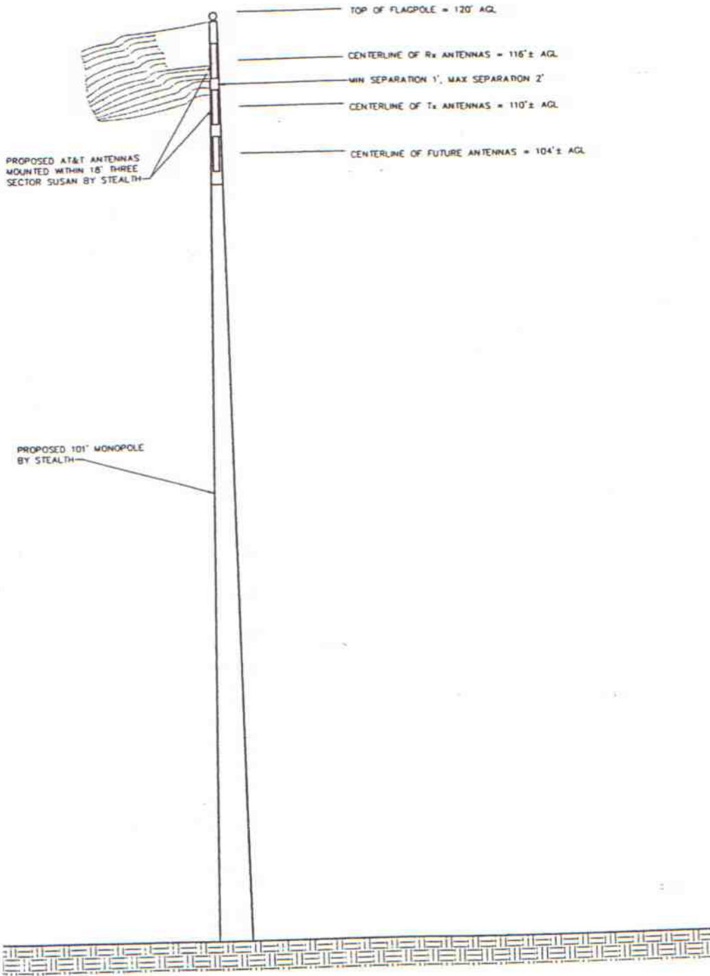
1 TOWER ELEVATION NO SCALE
